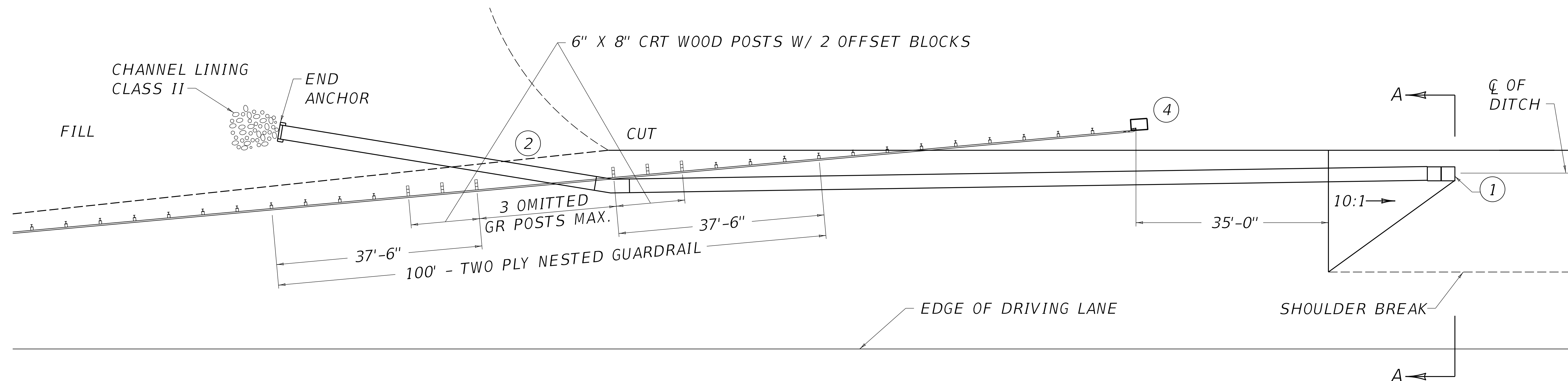
PLAN VIEW
